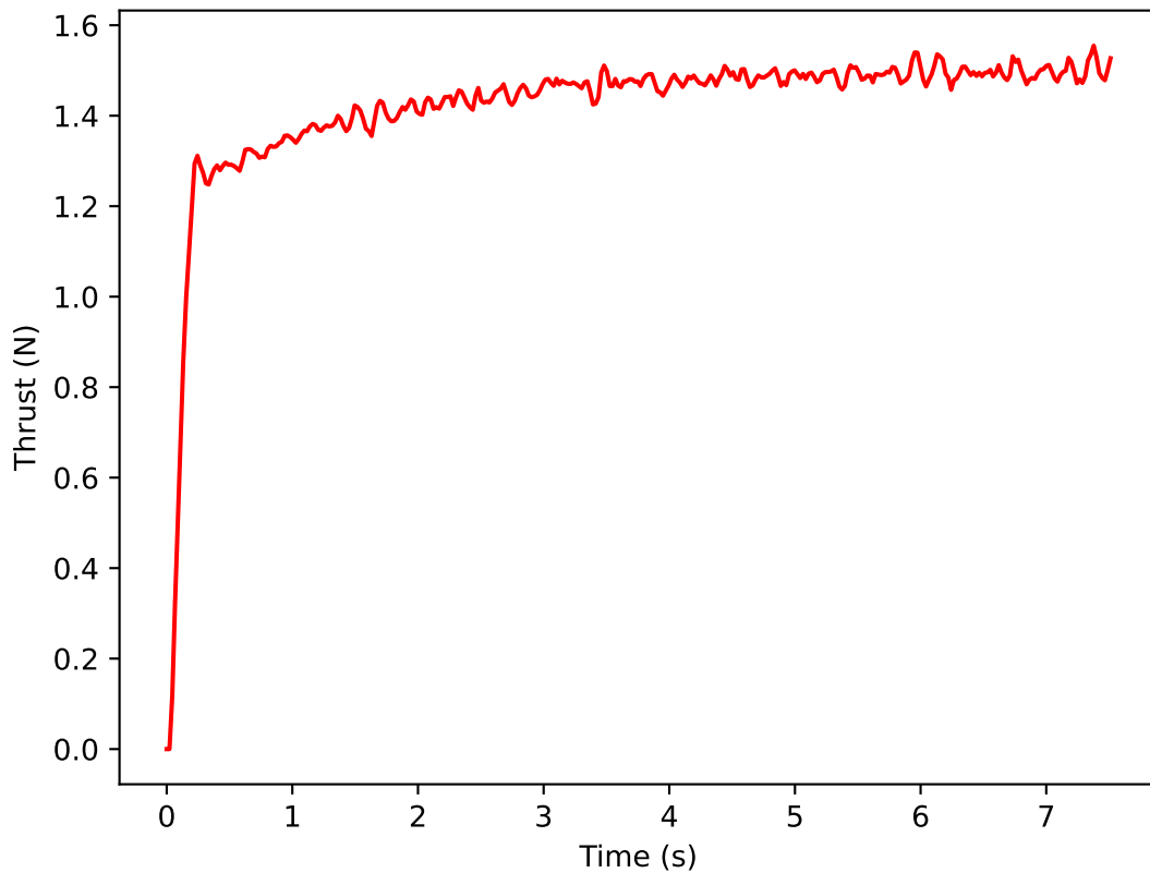
Takeoff Thrust Plot
